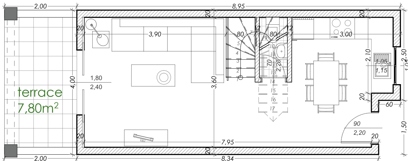
ground floor 34,84m 2
