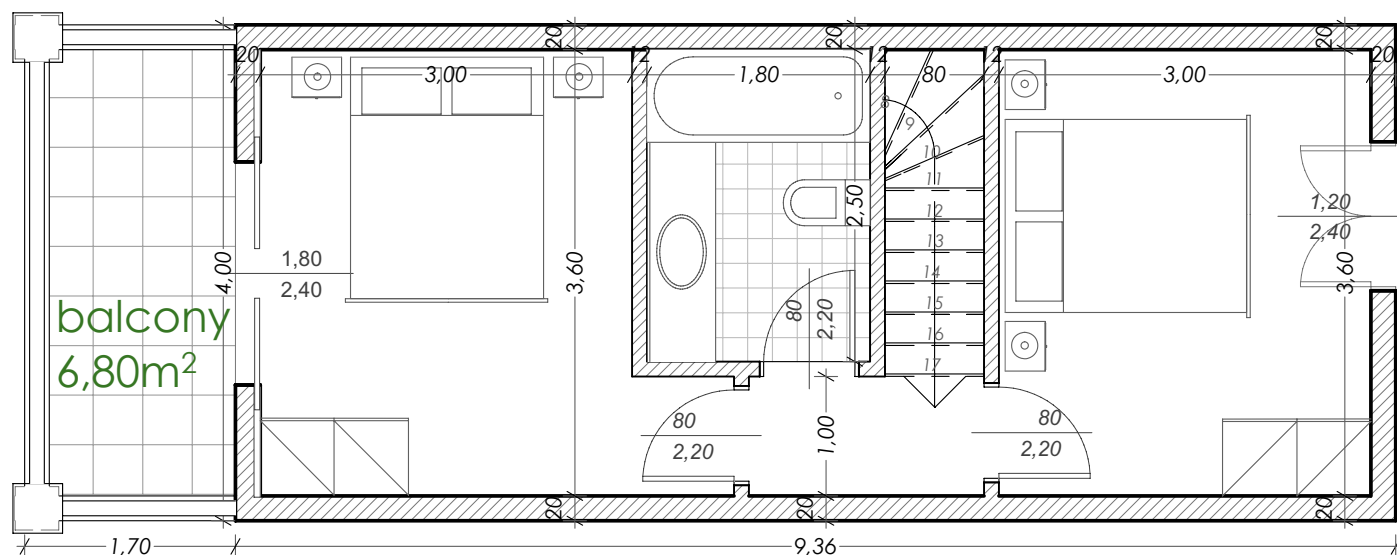
first floor 37,44m 2
